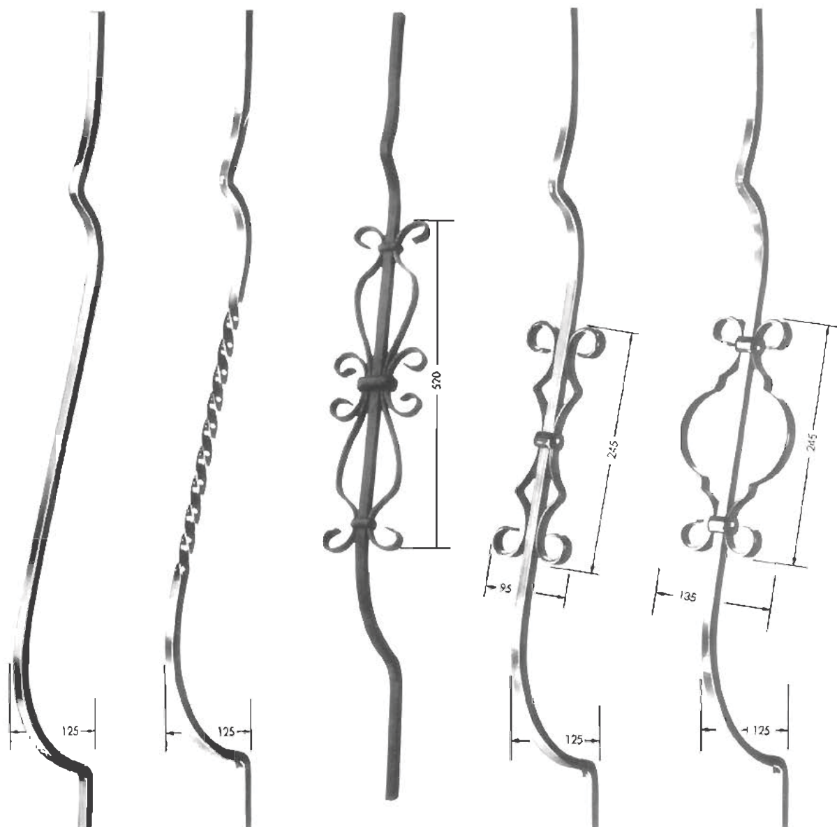
4-2094 L: 950 mm. Ø 12 mm.
